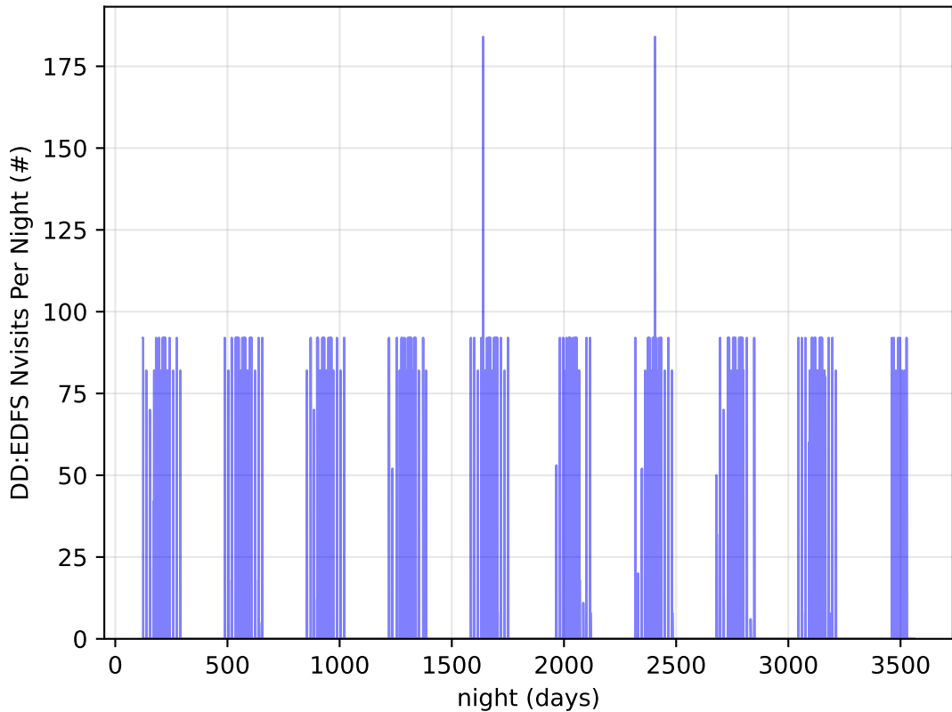
ddf_acor_sf25_lsf40_lsr20_v3.4_10yrs all bands: DD:EDFS Nvisits Per Night
