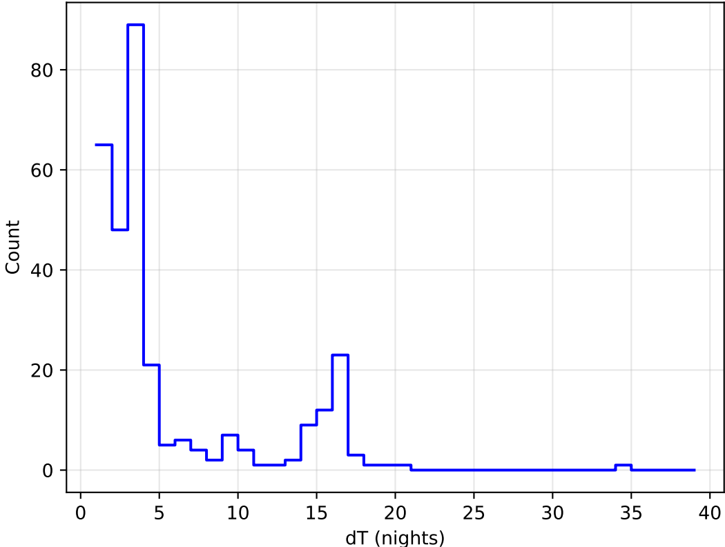
ddf_acor_sf25_Isf40_Isr20_v3.4_10yrs all bands: DD:EDFS Delta Nights Histogram
