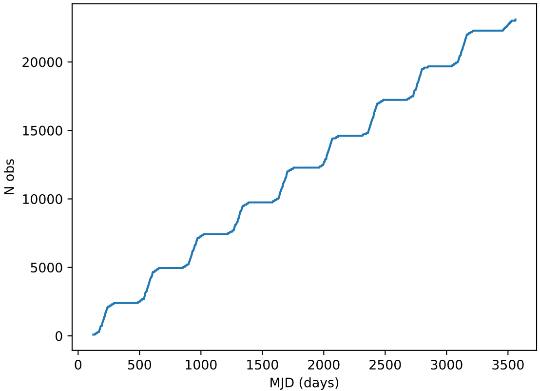
ddf_acor_sf25_lsf40_lsr20_v3.4_10yrs all bands: DD:EDFS Cumulative NVisits
