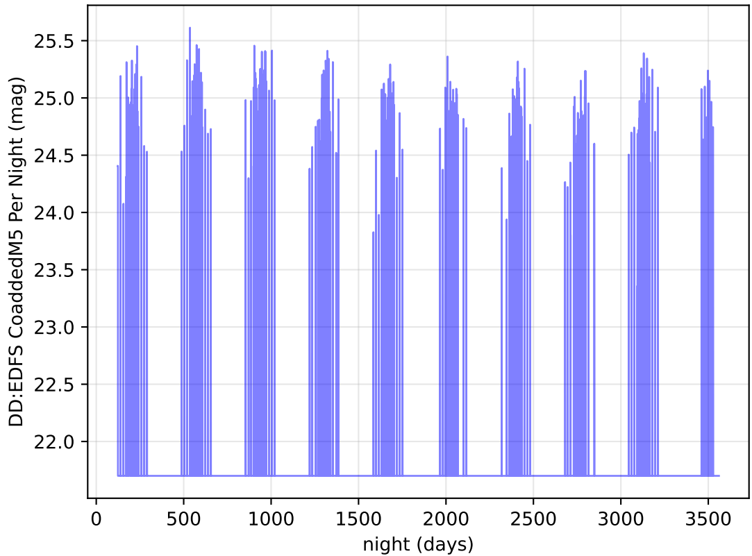
ddf_acor_sf25_lsf40_lsr20_v3.4_10yrs z band: DD:EDFS CoaddedM5 Per Night
