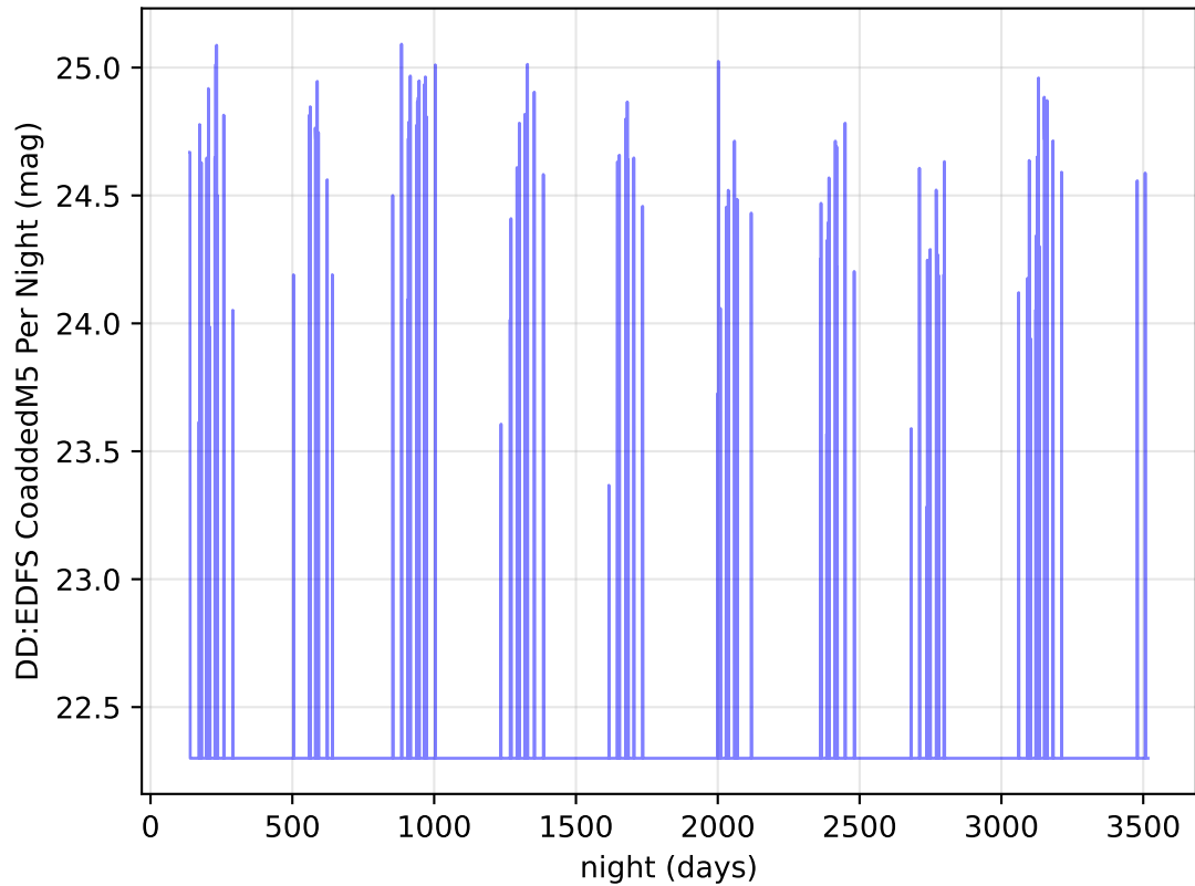
ddf_acor_sf25_lsf40_lsr20_v3.4_10yrs u band: DD:EDFS CoaddedM5 Per Night
