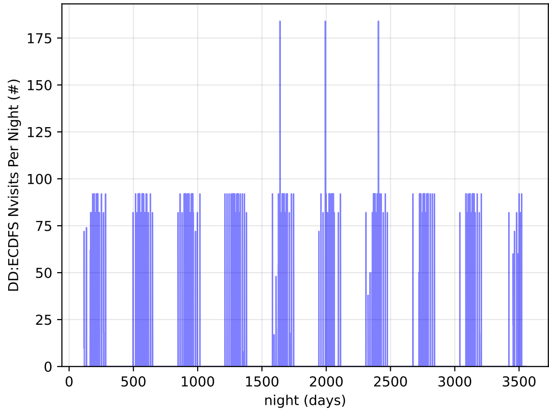
ddf_acor_sf25_lsf40_lsr20_v3.4_10yrs all bands: DD:ECDFS Nvisits Per Night
