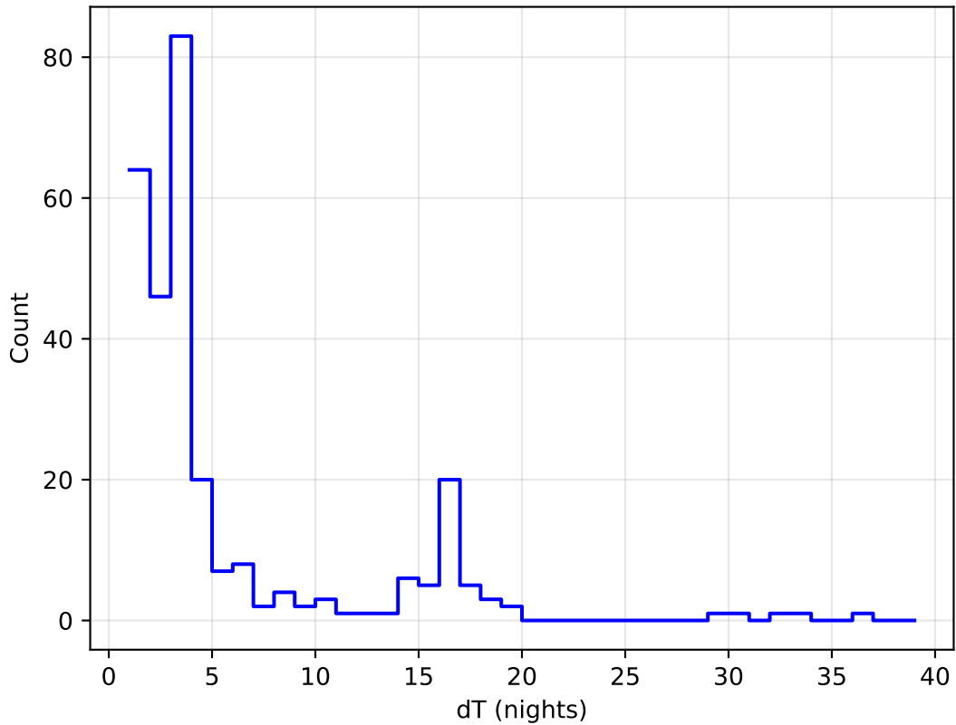
ddf_acor_sf25_lsf40_lsr20_v3.4_10yrs all bands: DD:ECDFS Delta Nights Histogram
