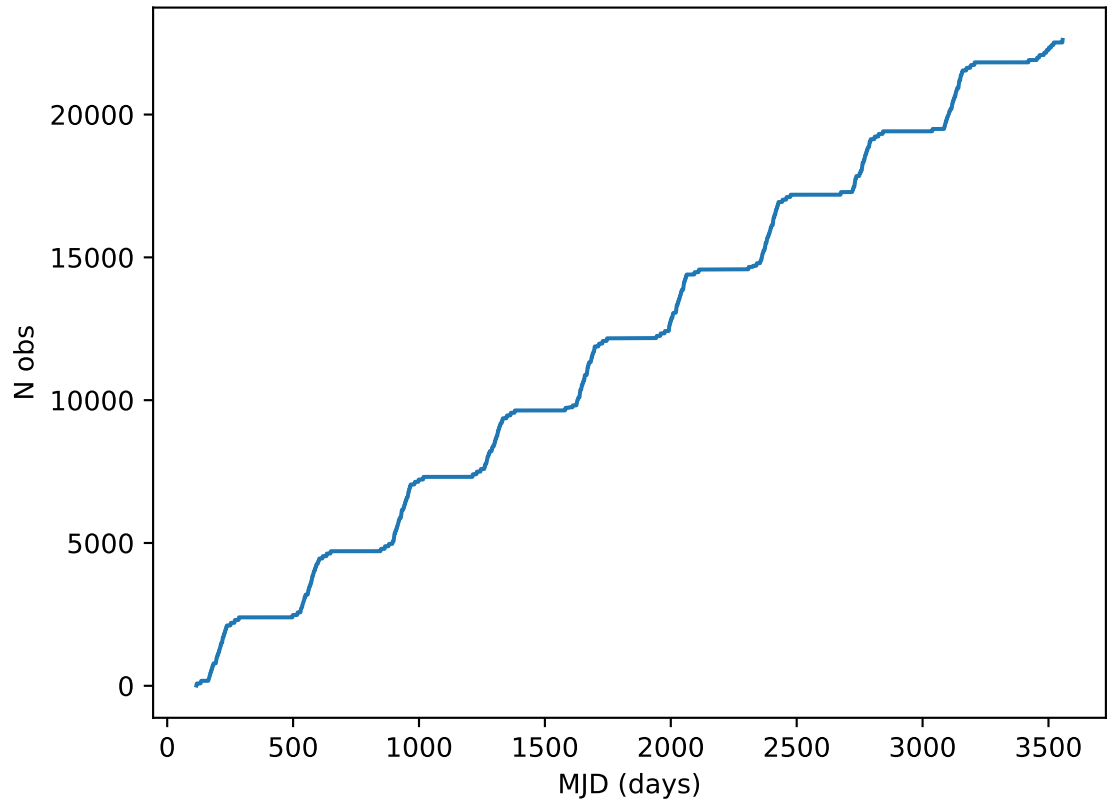
ddf_acor_sf25_lsf40_lsr20_v3.4_10yrs all bands: DD:ECDFS Cumulative NVisits
