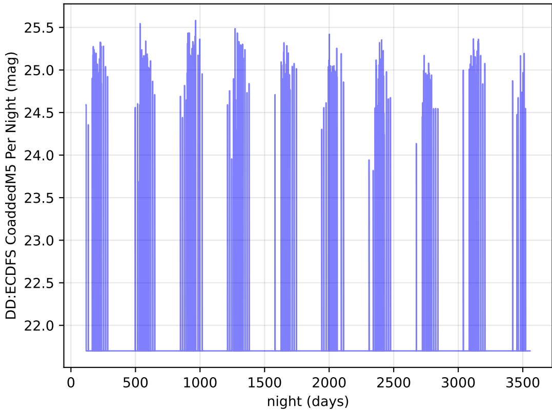
ddf_acor_sf25_lsf40_lsr20_v3.4_10yrs z band: DD:ECDFS CoaddedM5 Per Night
