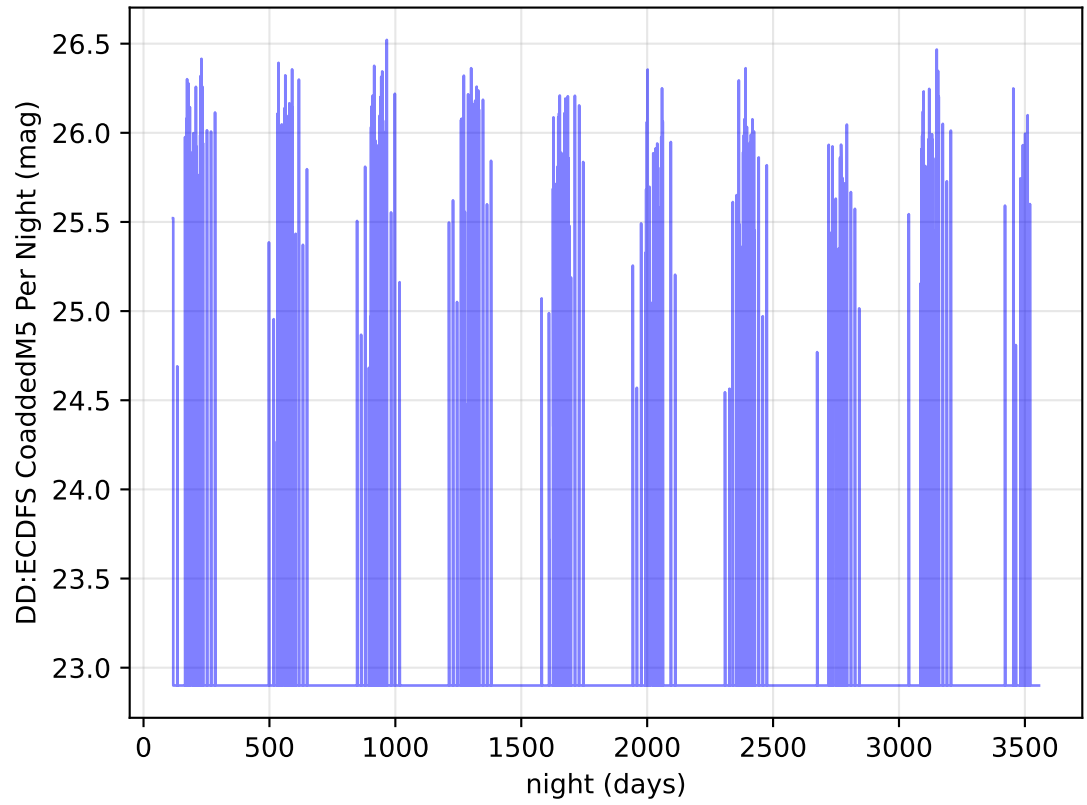
ddf_acor_sf25_lsf40_lsr20_v3.4_10yrs r band: DD:ECDFS CoaddedM5 Per Night
