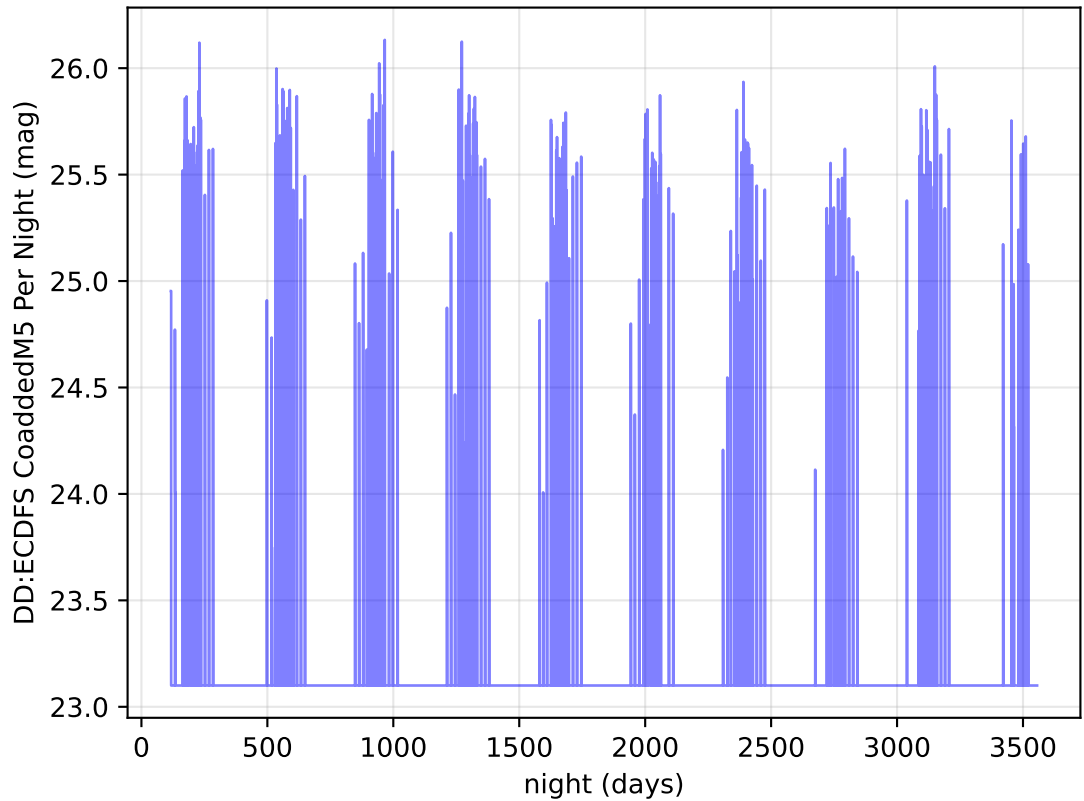
ddf_acor_sf25_lsf40_lsr20_v3.4_10yrs i band: DD:ECDFS CoaddedM5 Per Night
