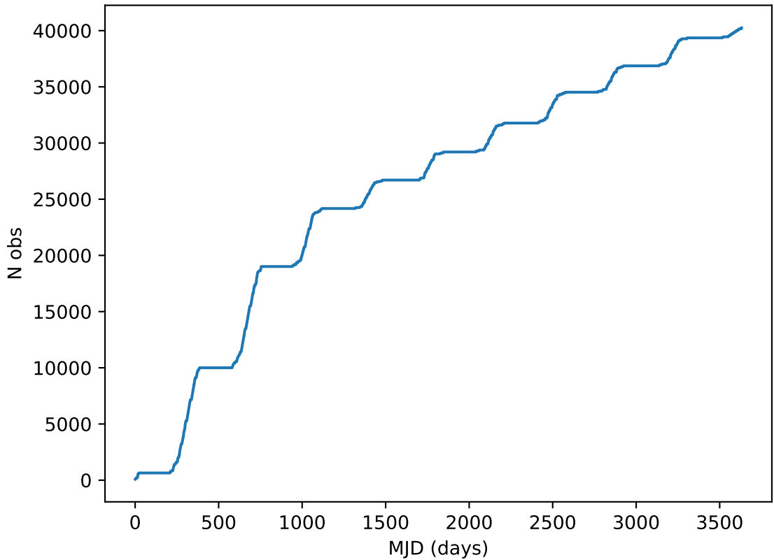
ddf_acor_sf25_lsf40_lsr20_v3.4_10yrs all bands: DD: COSMOS Cumulative NVisits
