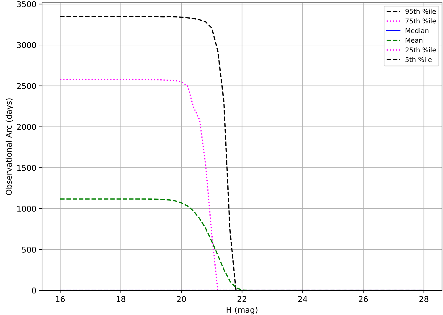
ddf_acor_sf25_lsf40_lsr10_v3.4_10yrs: Observational Arc Length Vatira
