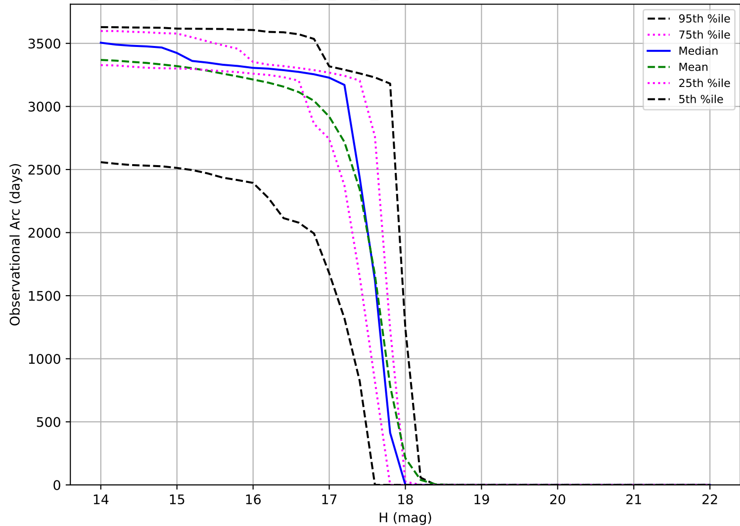
ddf_acor_sf25_lsf40_lsr10_v3.4_10yrs: Observational Arc Length Trojan
