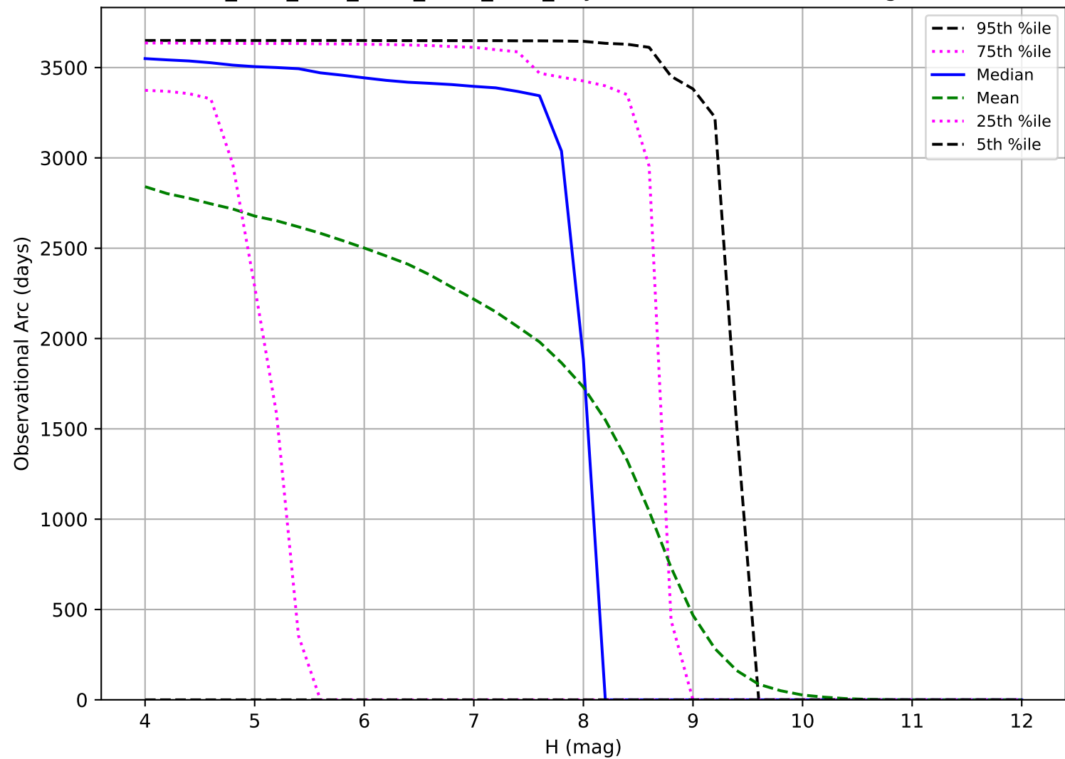
ddf_acor_sf25_Isf40_Isr10_v3.4_10yrs: Observational Arc Length TNO
