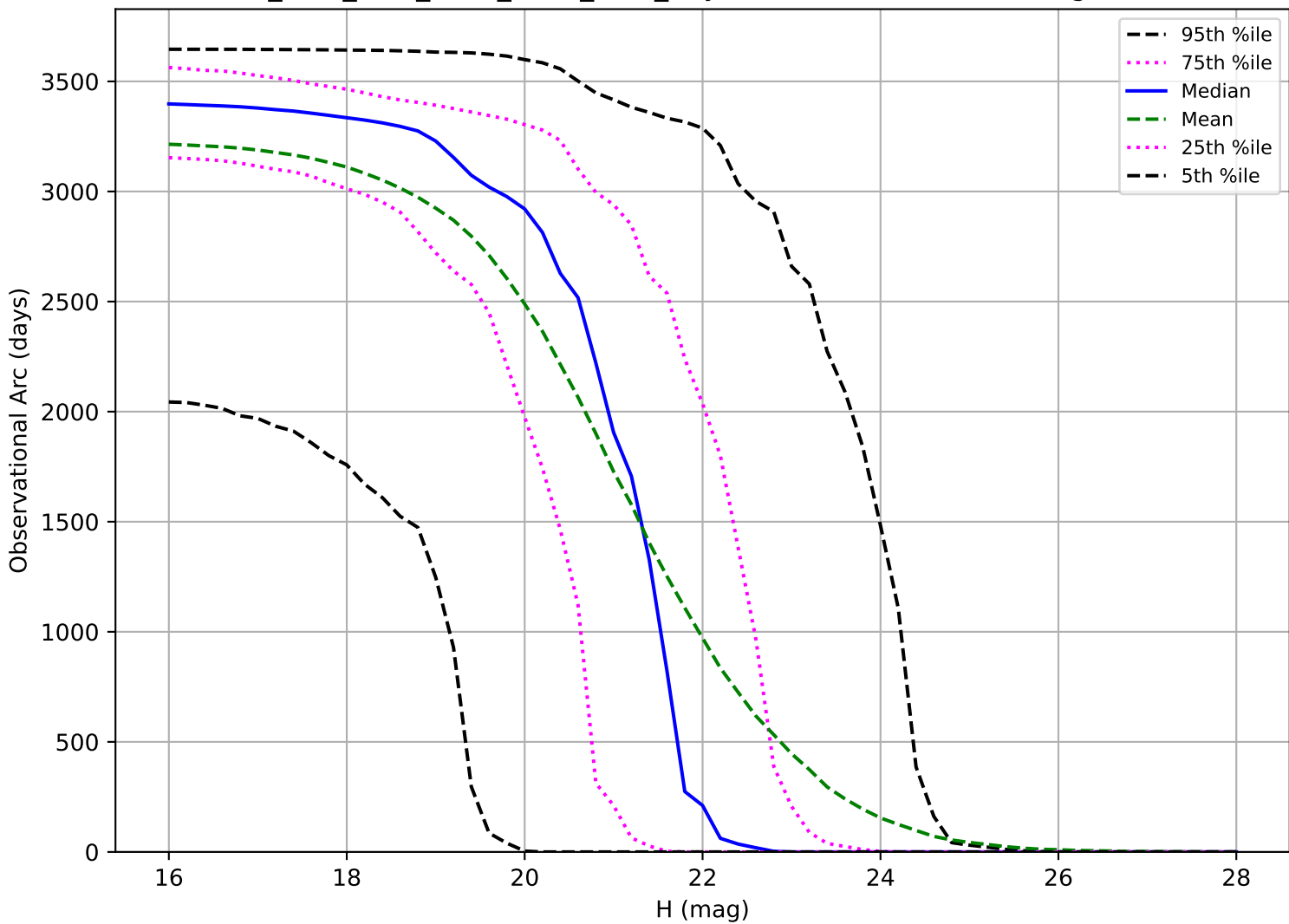
ddf_acor_sf25_lsf40_lsr10_v3.4_10yrs: Observational Arc Length PHA
