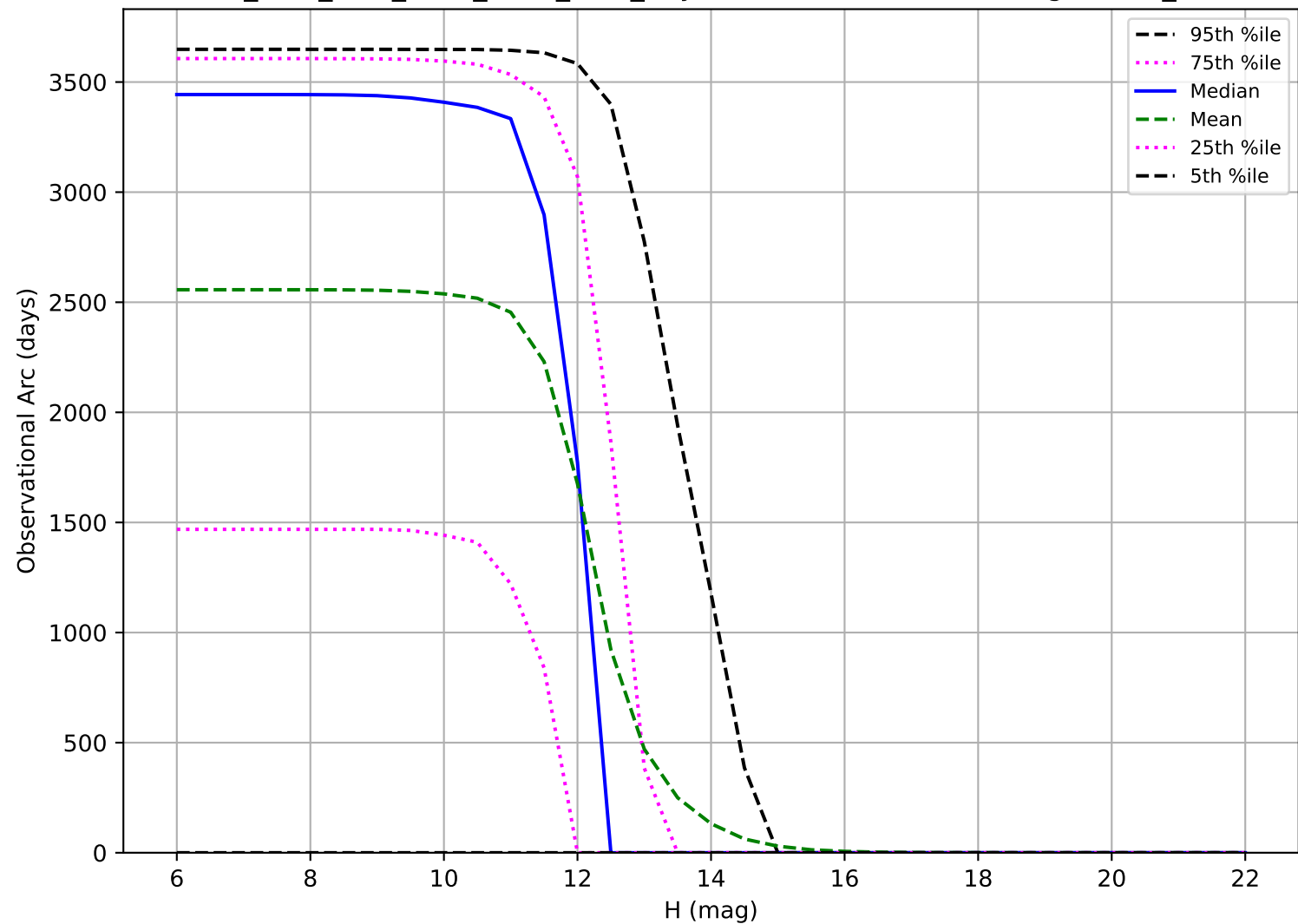
ddf_acor_sf25_lsf40_lsr10_v3.4_10yrs: Observational Arc Length OCC_r20
