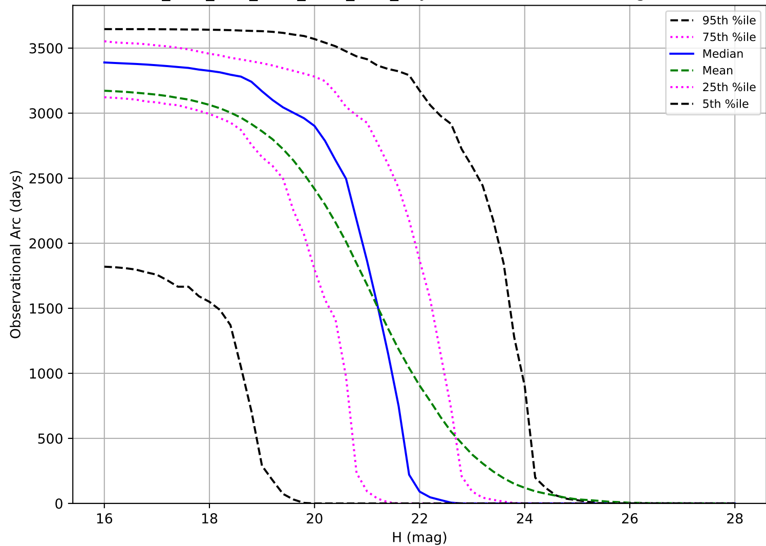
ddf_acor_sf25_lsf40_lsr10_v3.4_10yrs: Observational Arc Length NEO
