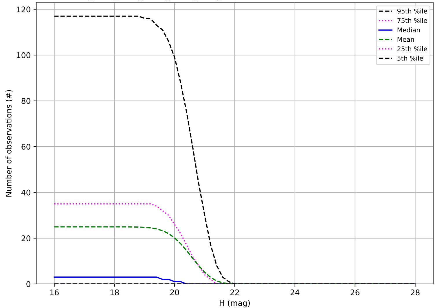
ddf_acor_sf25_lsf40_lsr10_v3.4_10yrs: Number of observations Vatira
