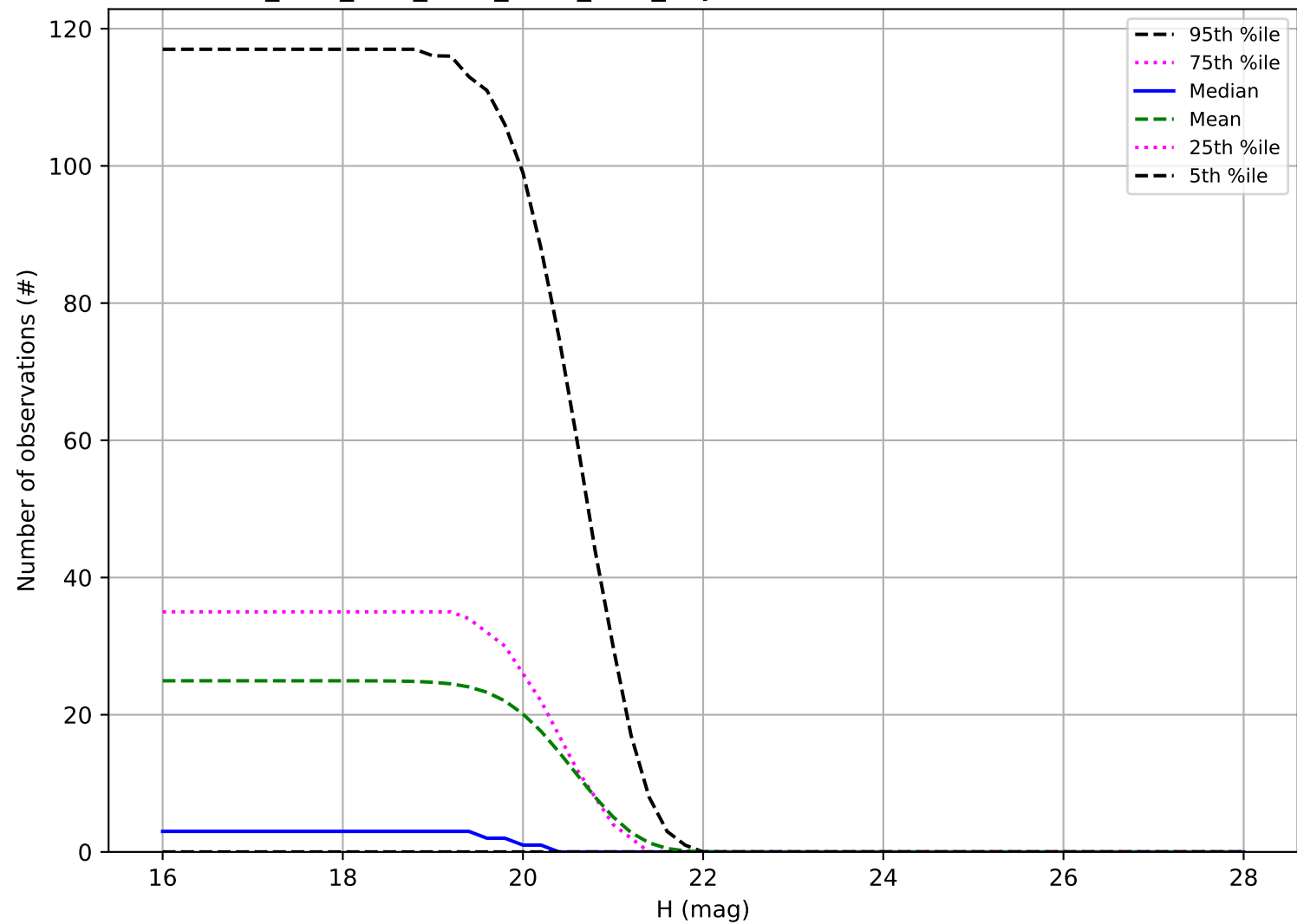
ddf_acor_sf25_lsf40_lsr10_v3.4_10yrs: Number of observations Vatira
