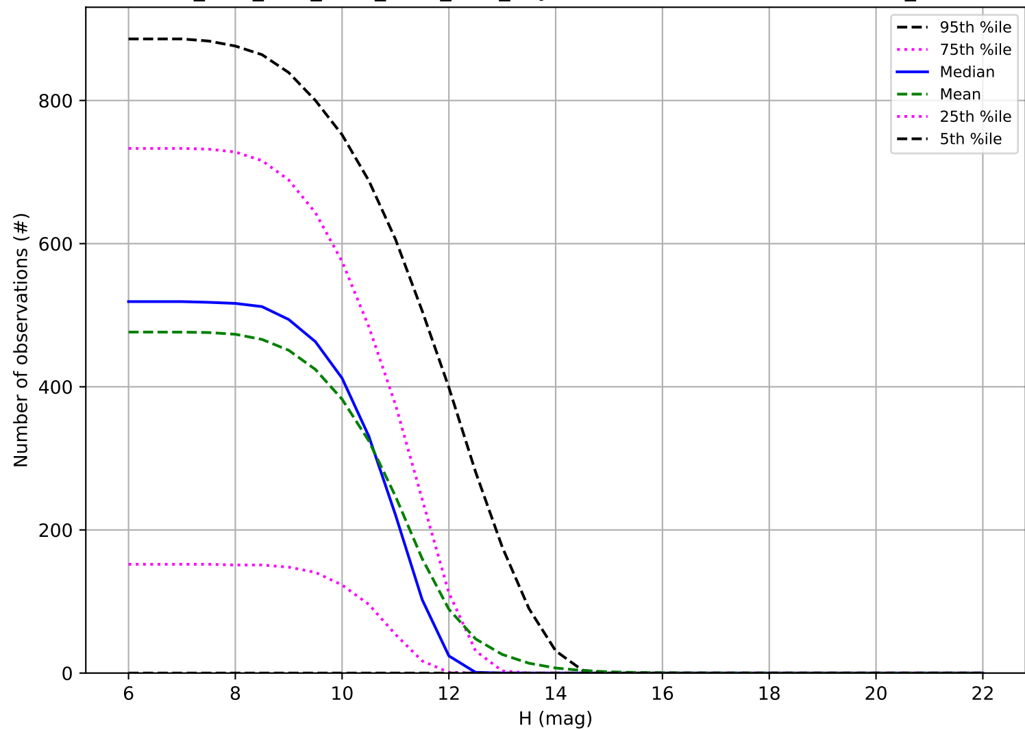
ddf_acor_sf25_lsf40_lsr10_v3.4_10yrs: Number of observations OCC_r20
