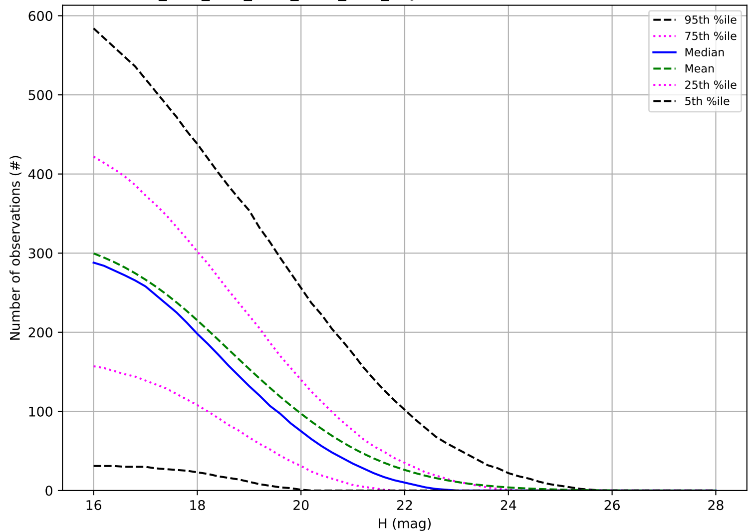
ddf_acor_sf25_lsf40_lsr10_v3.4_10yrs: Number of observations NEO
