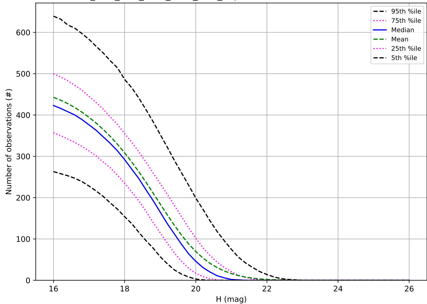
ddf_acor_sf25_lsf40_lsr10_v3.4_10yrs: Number of observations MBA
