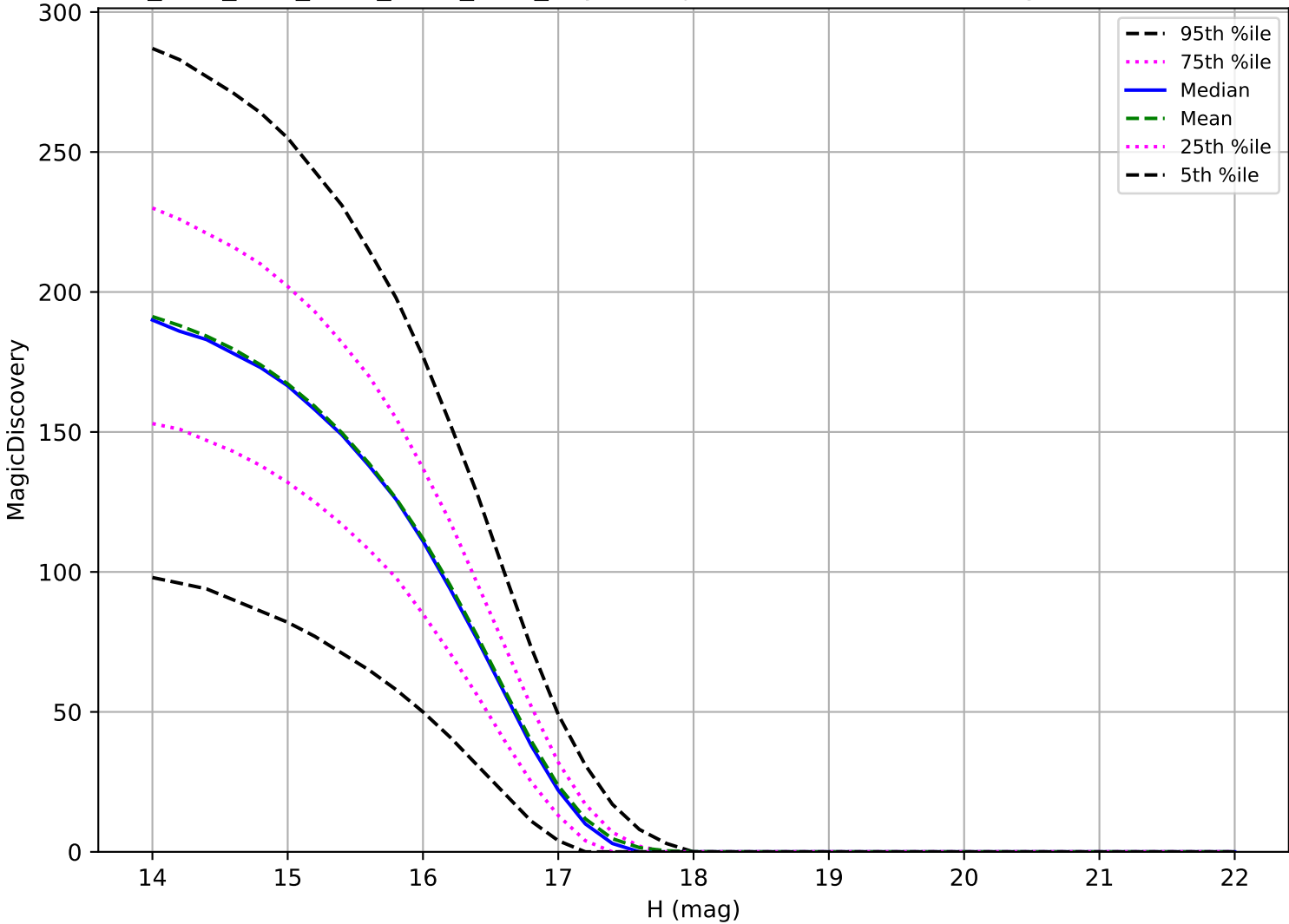
ddf_acor_sf25_lsf40_lsr10_v3.4_10yrs: Trojan 6 detections in 60 nights detection loss
