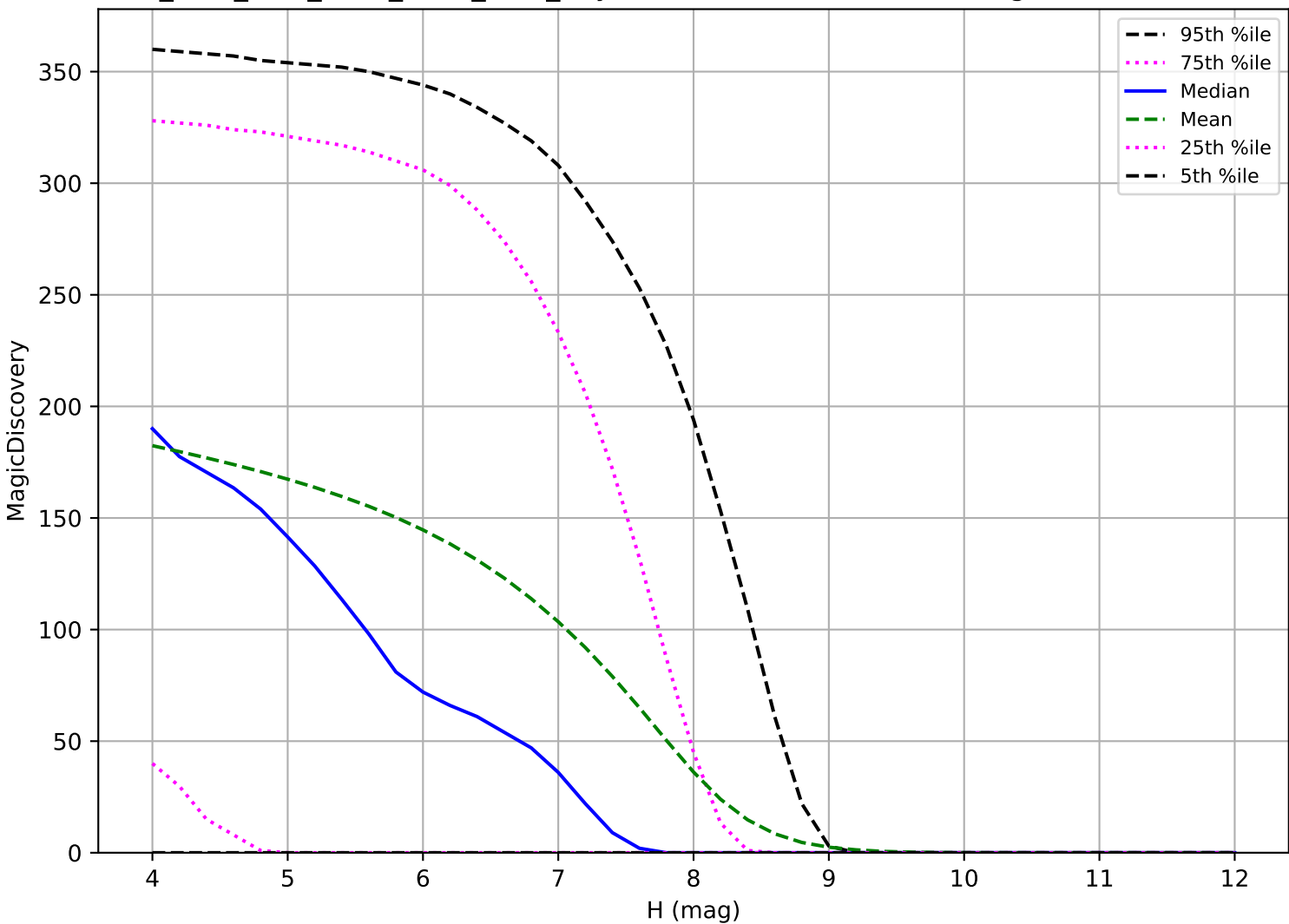
ddf_acor_sf25_lsf40_lsr10_v3.4_10yrs: TNO 6 detections in 60 nights detection loss
