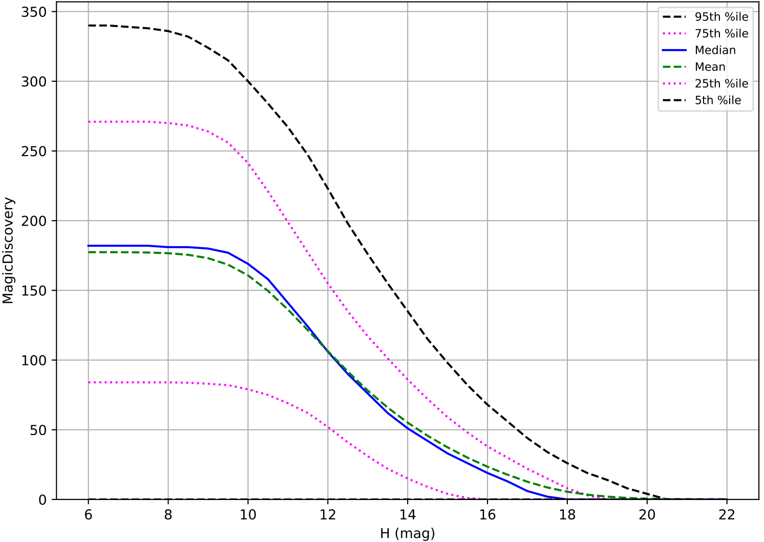
ddf_acor_sf25_lsf40_lsr10_v3.4_10yrs: OCC_r5 6 detections in 60 nights detection loss
