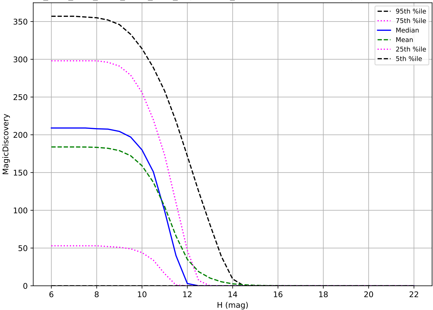
ddf_acor_sf25_lsf40_lsr10_v3.4_10yrs: OCC_r20 6 detections in 60 nights detection loss
