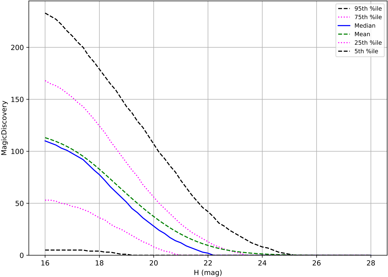
ddf_acor_sf25_lsf40_lsr10_v3.4_10yrs: NEO 6 detections in 60 nights detection loss
