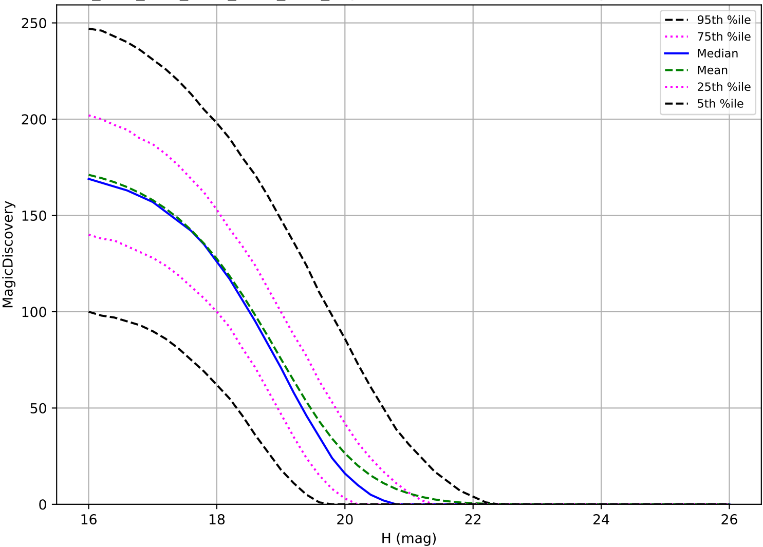
ddf_acor_sf25_lsf40_lsr10_v3.4_10yrs: MBA 6 detections in 60 nights detection loss
