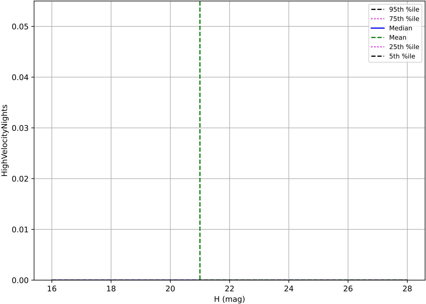
ddf_acor_sf25_lsf40_lsr10_v3.4_10yrs: Vatira High velocity pair detection loss
