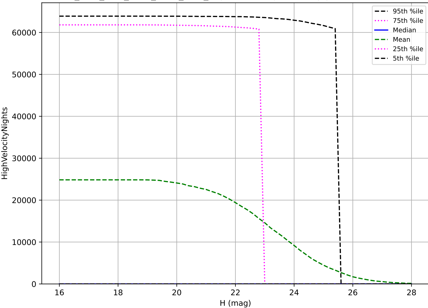
ddf_acor_sf25_lsf40_lsr10_v3.4_10yrs: PHA High velocity pair detection loss
