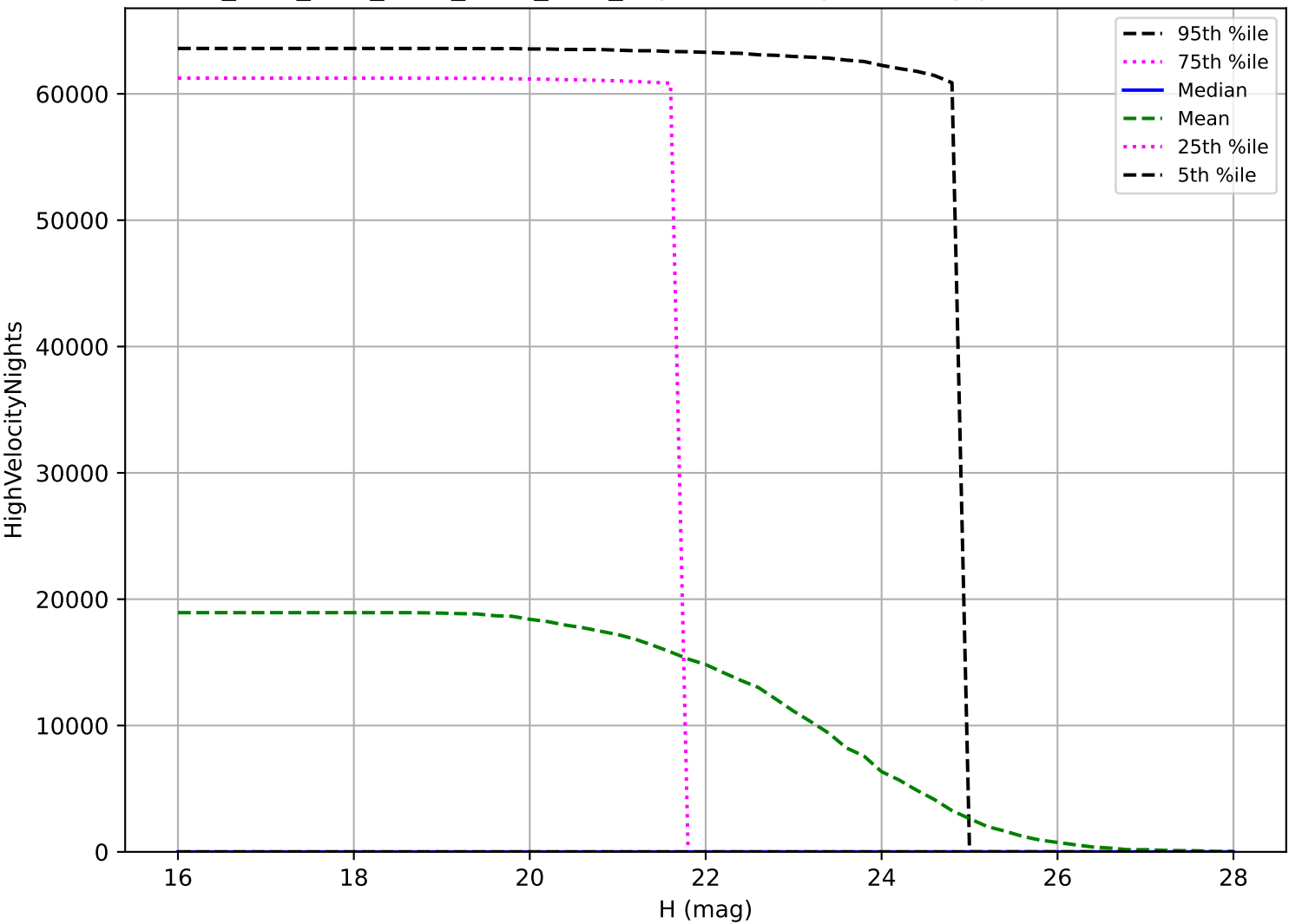
ddf_acor_sf25_lsf40_lsr10_v3.4_10yrs: NEO High velocity pair detection loss
