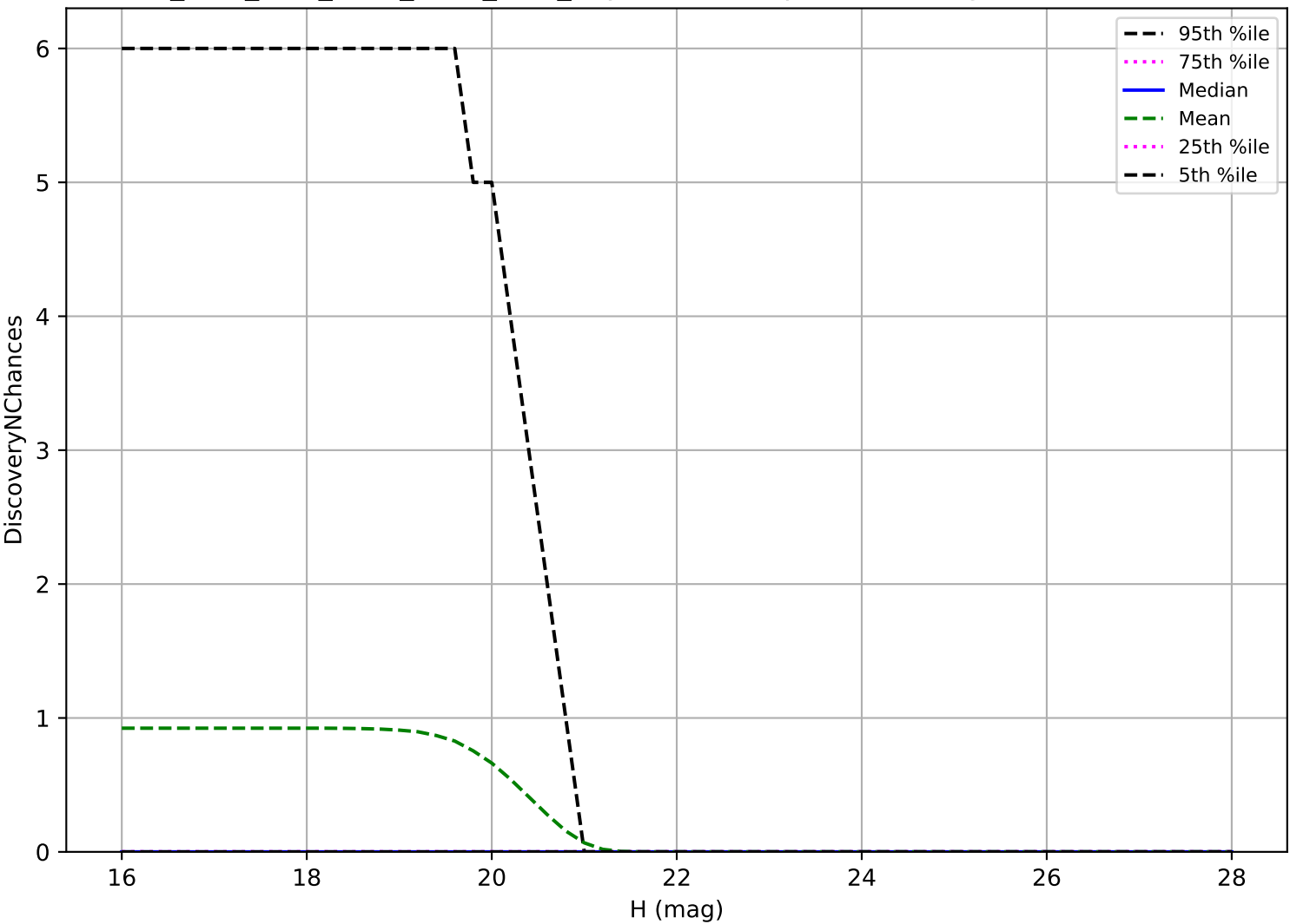
ddf_acor_sf25_lsf40_lsr10_v3.4_10yrs: Vatira 3 pairs in 15 nights detection loss
