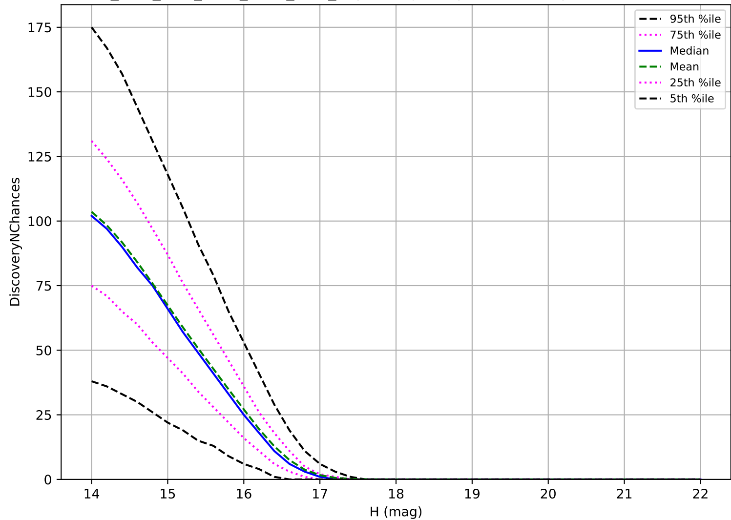
ddf_acor_sf25_lsf40_lsr10_v3.4_10yrs: Trojan 3 pairs in 15 nights detection loss
