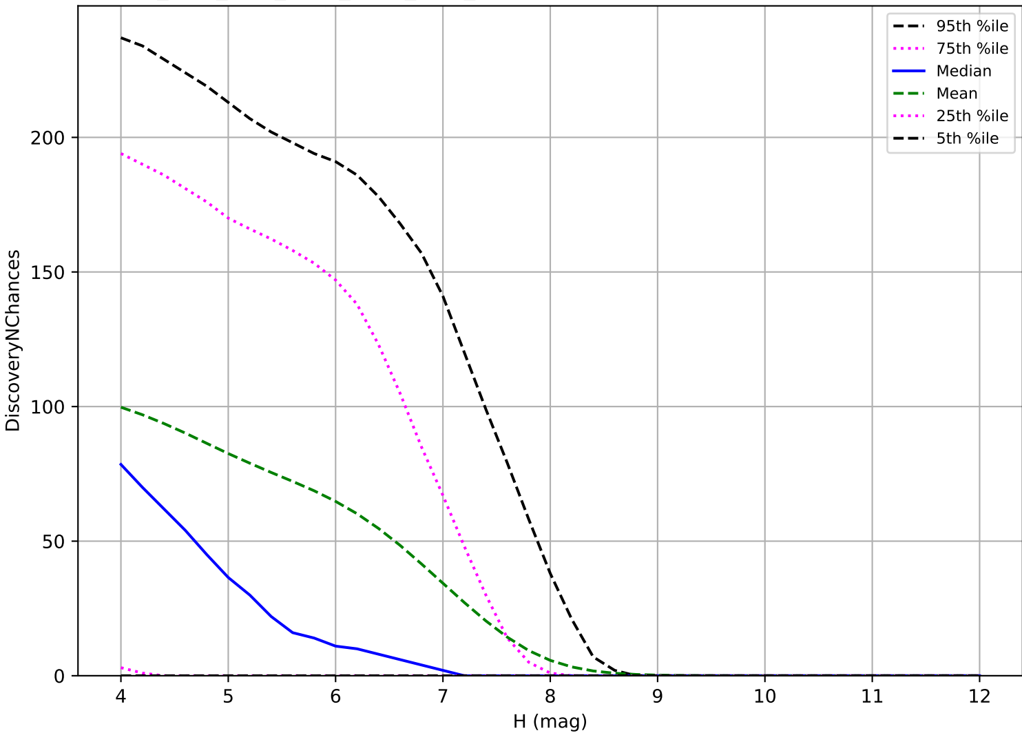
ddf_acor_sf25_lsf40_lsr10_v3.4_10yrs: TNO 3 pairs in 15 nights detection loss
