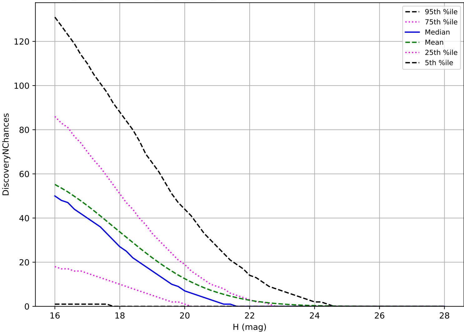
ddf_acor_sf25_lsf40_lsr10_v3.4_10yrs: PHA 3 pairs in 15 nights detection loss
