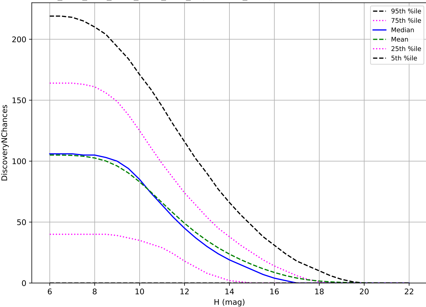
ddf_acor_sf25_lsf40_lsr10_v3.4_10yrs: OCC_r5 3 pairs in 15 nights detection loss
