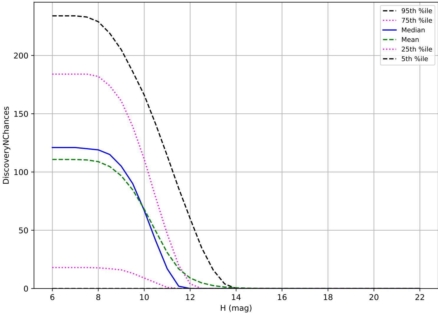
ddf_acor_sf25_lsf40_lsr10_v3.4_10yrs: OCC_r20 3 pairs in 15 nights detection loss
