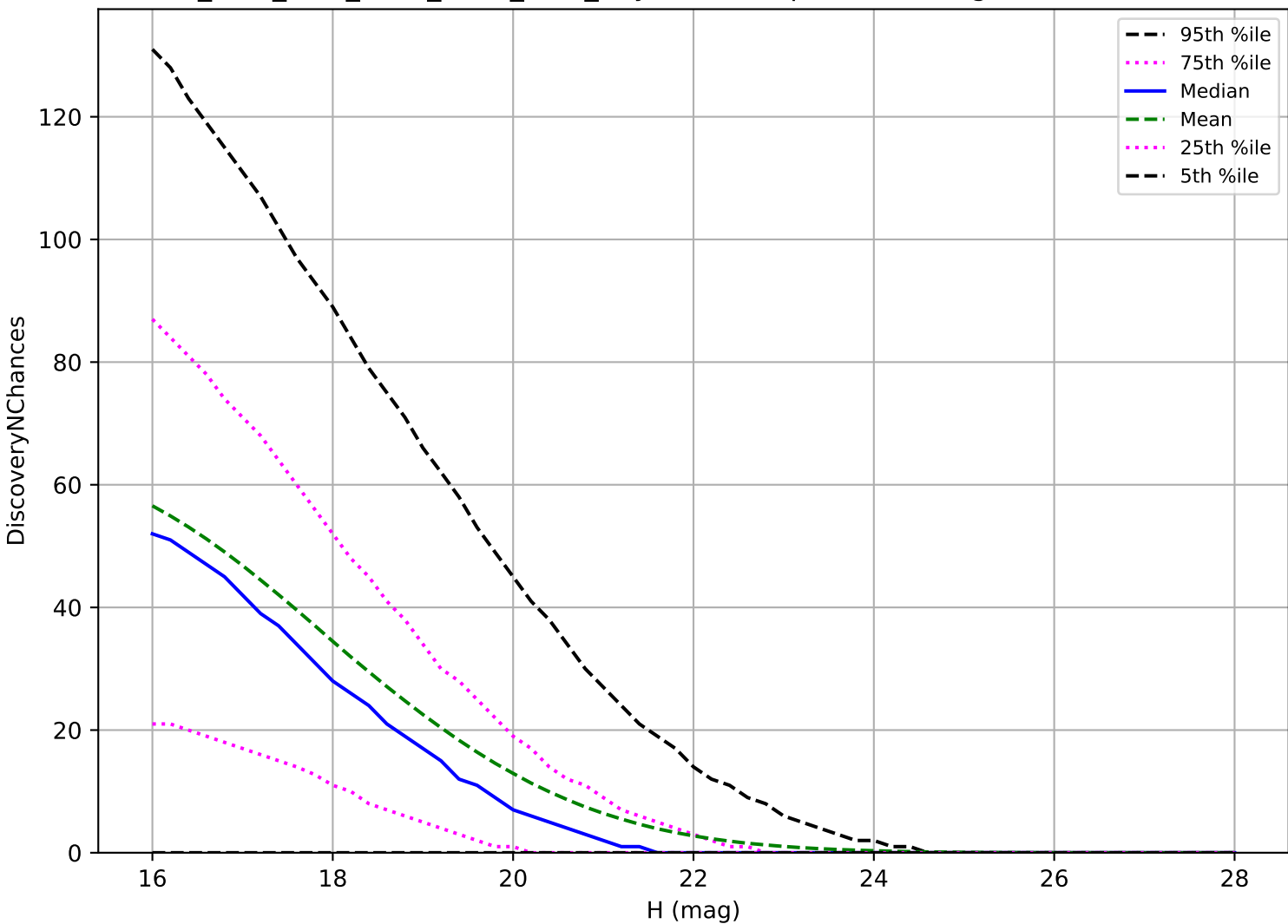
ddf_acor_sf25_lsf40_lsr10_v3.4_10yrs: NEO 3 pairs in 15 nights detection loss
