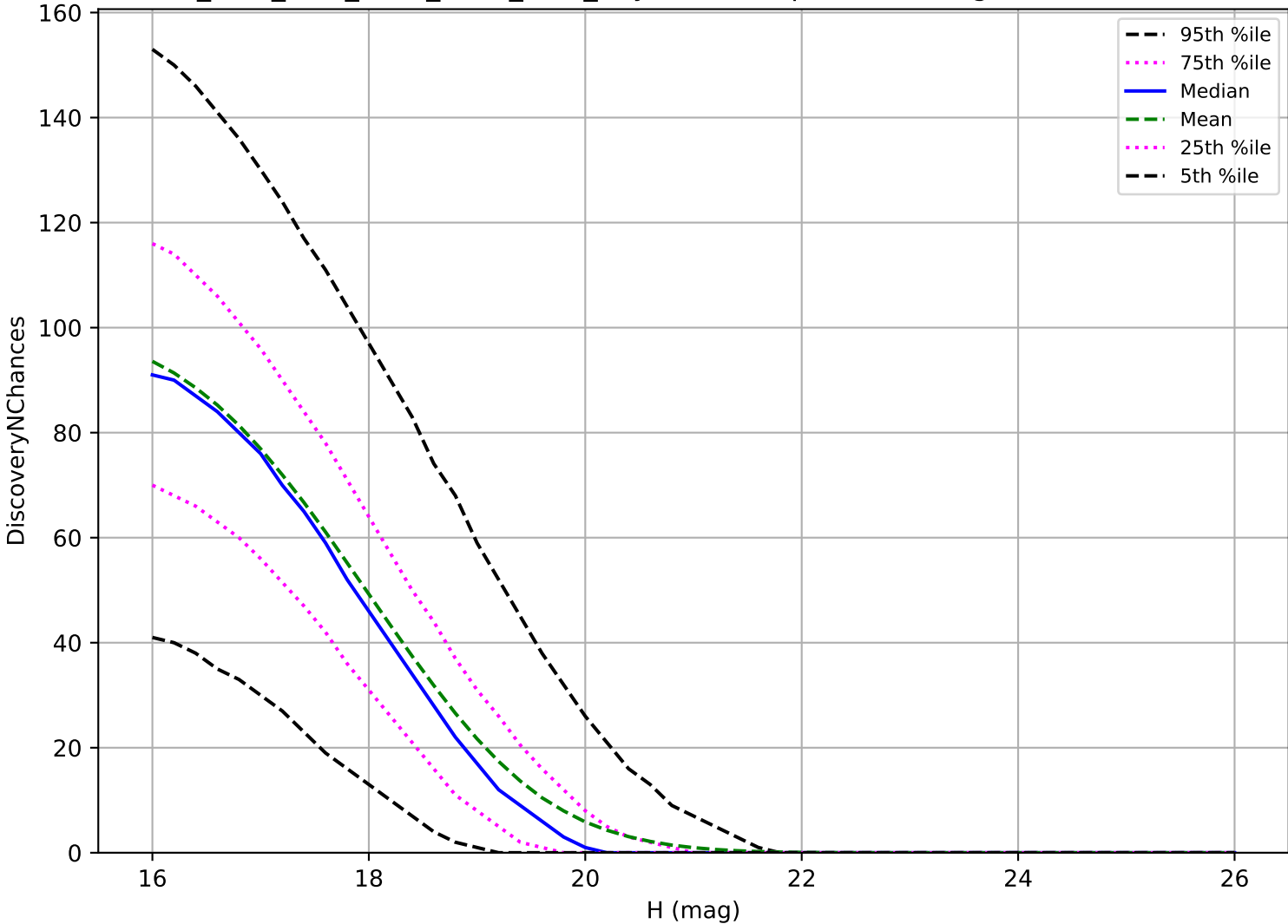
ddf_acor_sf25_lsf40_lsr10_v3.4_10yrs: MBA 3 pairs in 15 nights detection loss
