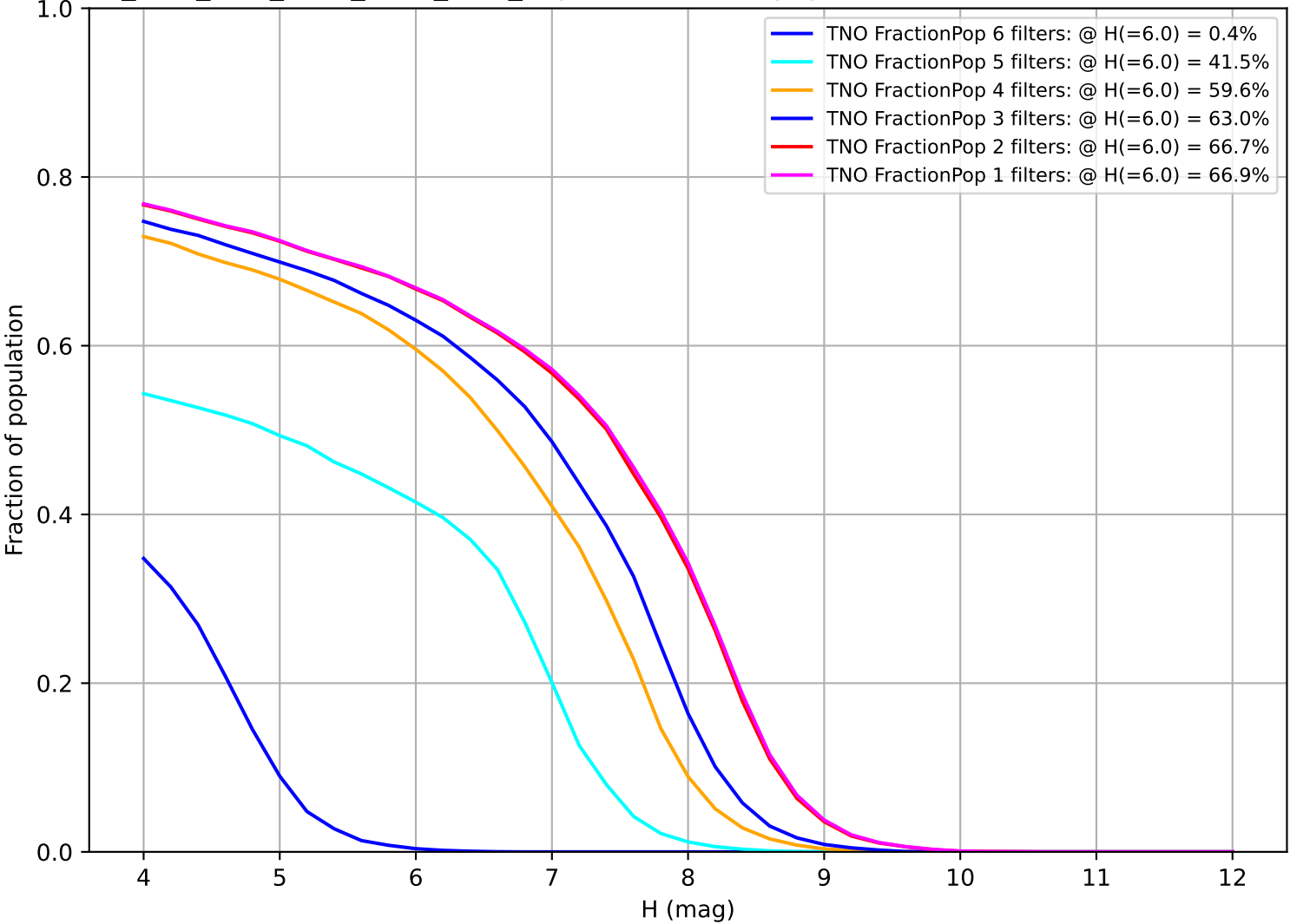
ddf_acor_sf25_lsf40_lsr10_v3.4_10yrs: Fraction of population with colors in X filters TNO
