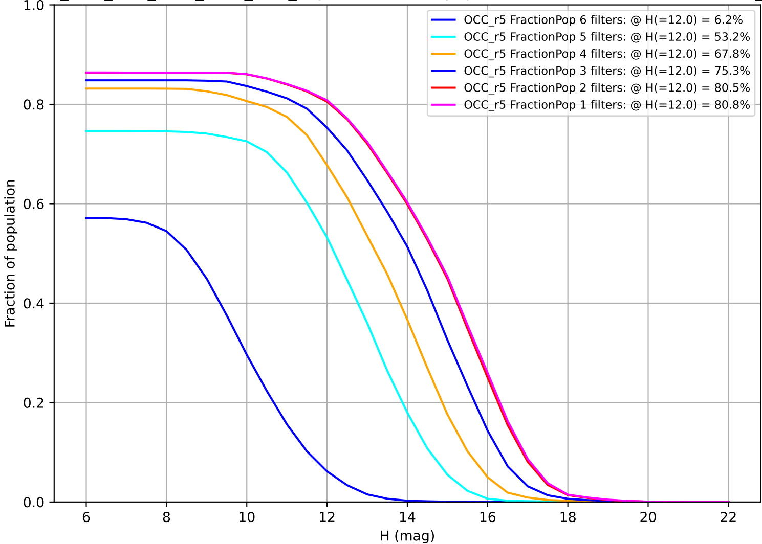
ddf_acor_sf25_lsf40_lsr10_v3.4_10yrs: Fraction of population with colors in X filters OCC_r5
