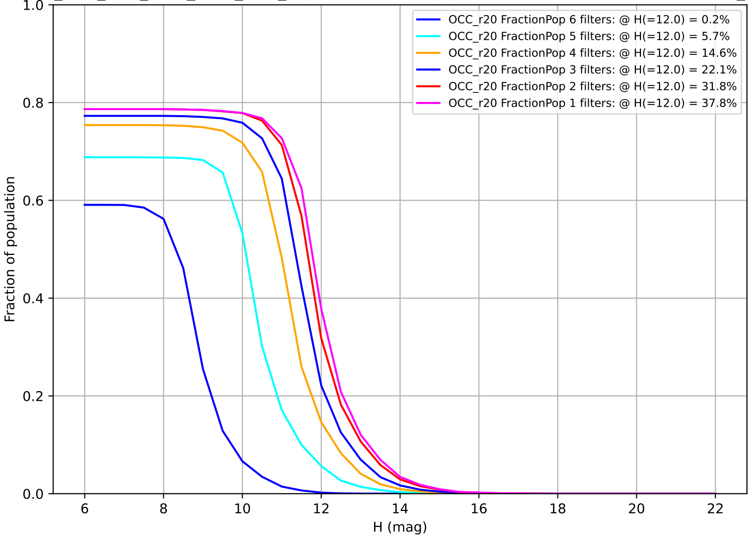
ddf_acor_sf25_lsf40_lsr10_v3.4_10yrs: Fraction of population with colors in X filters OCC_r20
