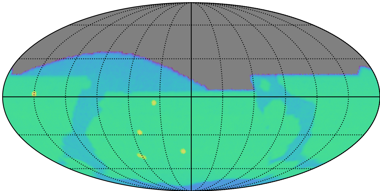
ddf_acor_sf25_lsf40_lsr10_v3.4_10yrs i: SurfaceBrightLimit
