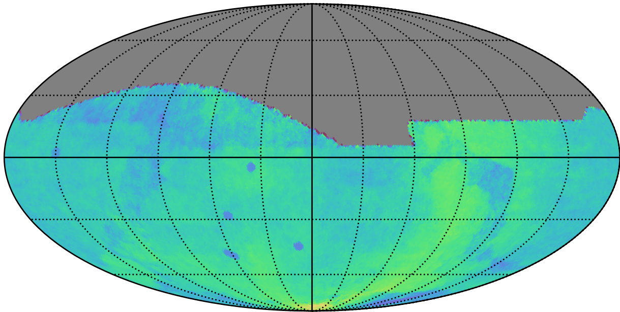
ddf_acor_sf25_lsf40_lsr10_v3.4_10yrs : Parallax Coverage @ 22.4
