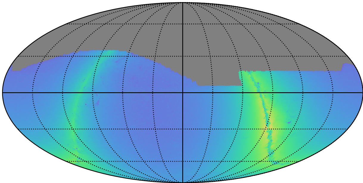
ddf_acor_sf25_lsf40_lsr10_v3.4_10yrs r: Nstars_no_crowding
