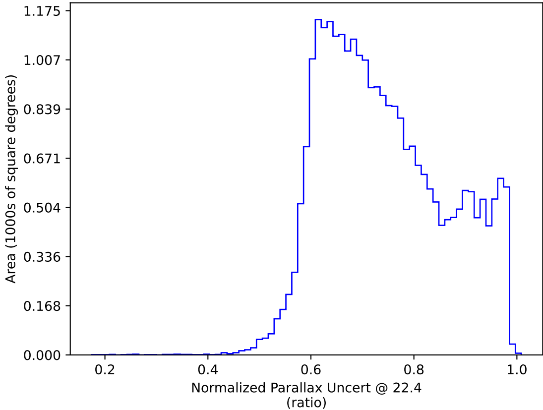
ddf_acor_sf25_lsf40_lsr10_v3.4_10yrs : Normalized Parallax Uncert @ 22.4
