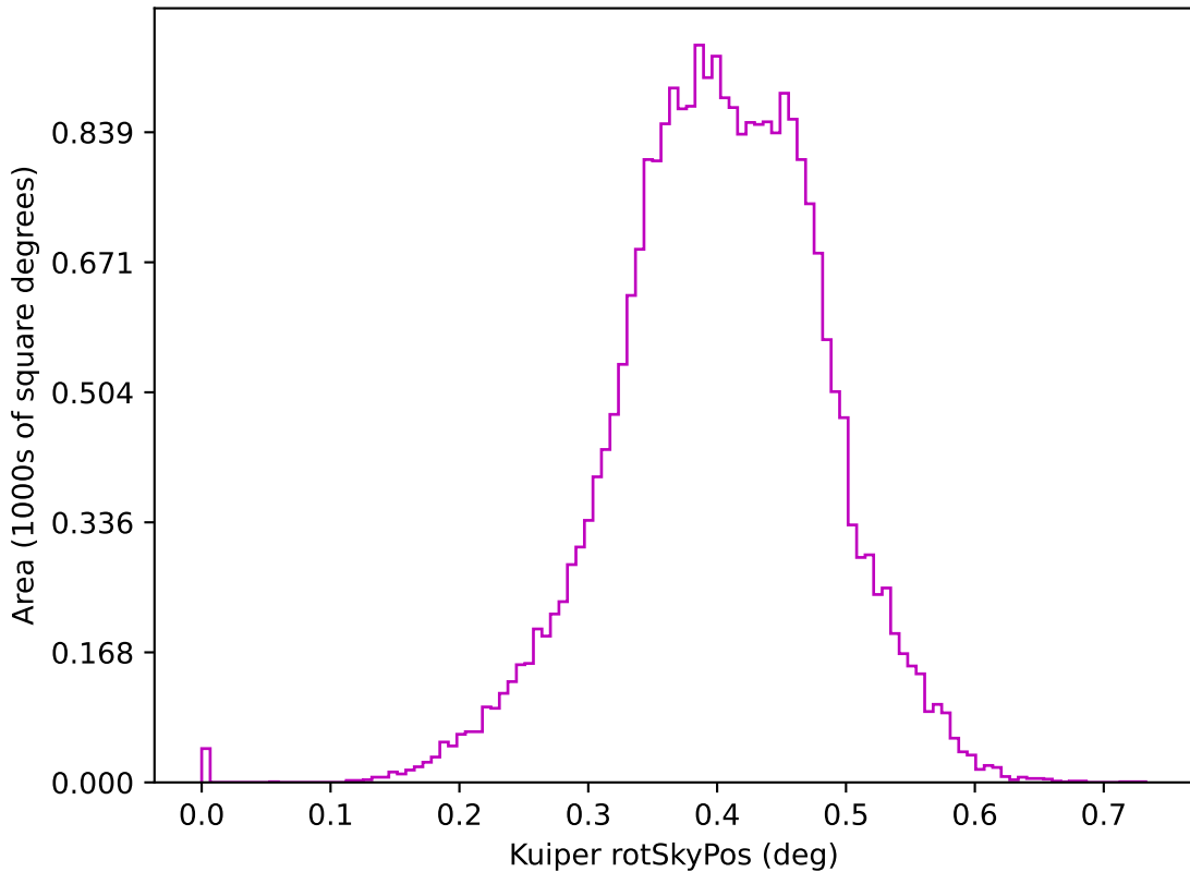
ddf_acor_sf25_lsf40_lsr10_v3.4_10yrs z: Kuiper rotSkyPos
