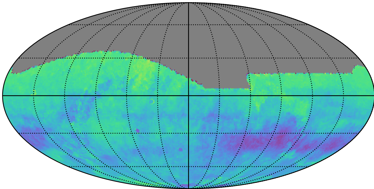
ddf_acor_sf25_lsf40_lsr10_v3.4_10yrs r: Kuiper rotSkyPos
