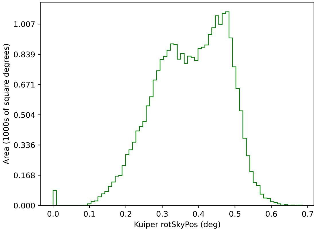
ddf_acor_sf25_lsf40_lsr10_v3.4_10yrs g: Kuiper rotSkyPos
