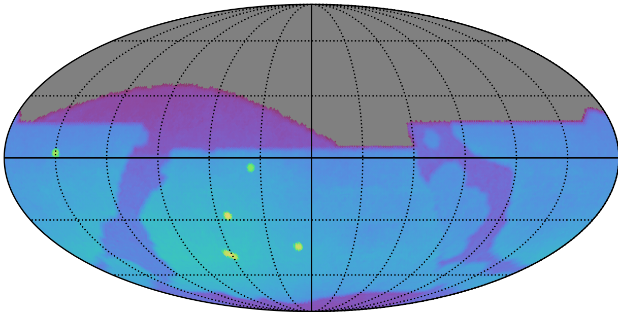
ddf_acor_sf25_lsf40_lsr10_v3.4_10yrs : Brown Dwarf, L4
